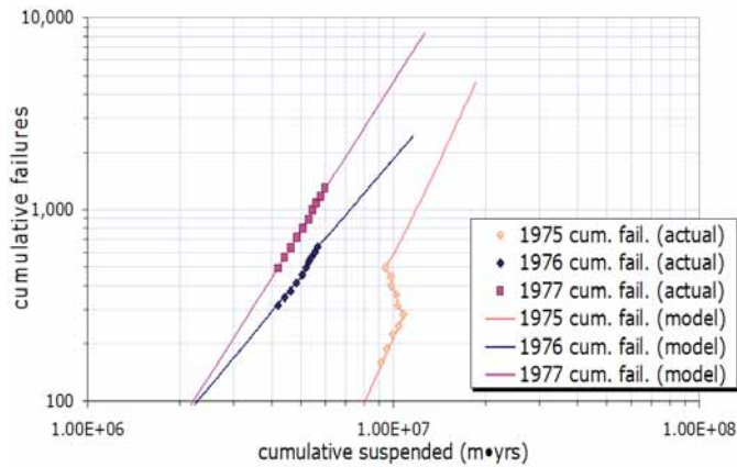
Figure 3. 1975-77 data and C-A models. The least squares slope ( \beta ), intercept ( \lambda ), and correlation coefficient ( r^2 ) are: 1975: 3.6, 2.19 \times 10^{-25} , 0.997; 1976: 1.9, 6.97 \times 10^{-12} , 0.996; 1977: 2.5, 6.00 \times 10^{-16} , 0.999.
