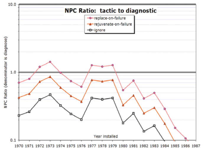
Figure 9. The ratio of net present costs of several tactical alternatives to diagnostic testing demonstrate testing almost always fails to meet the economic horizon criterion.
